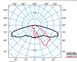
Publisca P1W-AB2L-LRA/1500-730 2G1S
