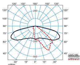
Cuvia60-AB2L12LA-S2-135-727-ET-CAB-26 (CLO end value)
