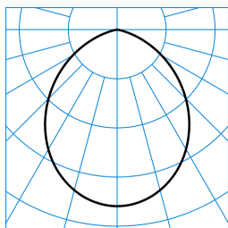
Skeo Q-W2 GS RB18R-RB18R/950-840 (direct) TX084366 ■ C0 - C180
