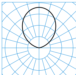
Skeo Q-W2 GS RB18R-RB18R/950-840 (indirect) TX084367 ■ C0 - C180
