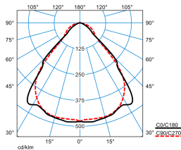
SFlow D3-L MRW LED4000-8TW ETDD8 LLWM 03 (DCW)
