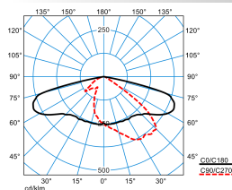
LIQ 70N-AB7L-LRA/9100-722 10G1 ETDD (CLO initial value)
