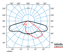
LIQ 70N-AB7L-LRA/9100-722 10G1 ETDD (CLO end value)
