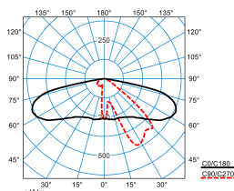
Publisca P1-AB2L-LRA/1650-740 2G1S ET (CLO end value) TX300692 DIN 5040: A30 UTE: 1,00 G DLOR: 100 % ULOR: 0 % CEN Flux Code: 34 70 96 100 100
