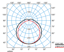
Deveo G3 6 DL 10-30/3ML-8MC ET PC +LV (stage 4)
