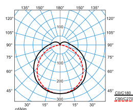
Deveo G3 6 DL 10-30/3ML-8MC ET PC +LV (stage 2)
