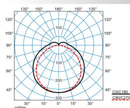
Deveo G3 6 DL 10-30/3ML-8MC ET PC +LV (stage 1)
