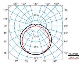
Deveo G3 6 DL 10-30/3ML-8MC ET PC +LV (stage 6)
