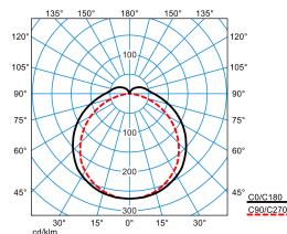
Deveo G3 6 DL 10-30/3ML-8MC ET PC +LV (stage 3)
