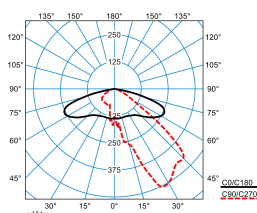
Publisca P2-AB2L-LRA/2900-740 4G1S ET (CLO initial value) TX300909 DIN 5040: A30 UTE: 1,00 G DLOR: 100 % ULOR: 0 % CEN Flux Code: 35 73 97 100 100
