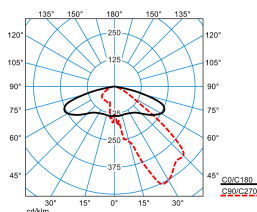
Publisca P2-AB2L-LRA/2900-740 4G1S ET (CLO end value) TX301695 DIN 5040: A30 UTE: 1,00 G DLOR: 100 % ULOR: 0 % CEN Flux Code: 35 73 97 100 100
