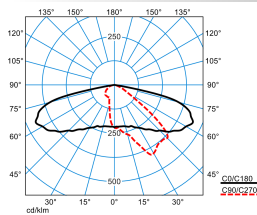
LIQ 50N-AB2L-LRA/2200-740 2G1 ETDD (CLO initial value)
