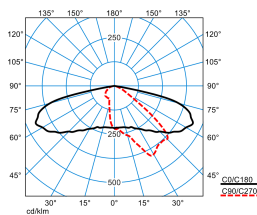
LIQ 50N-AB2L-LRA/2200-740 2G1 ETDD (CLO end value)
