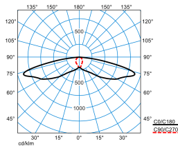
LIQ 50N-SB3L-LR/1200-727 2G1 ET (CLO end value) TX779561
