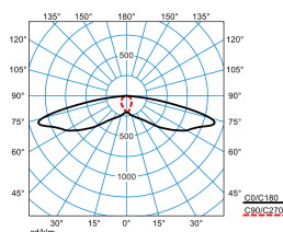
LIQ 50N-SB3L-LR/1200-727 2G1 ET (CLO end value)
