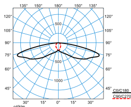
LIQ 50N-SB3L-LR/1200-727 2G1 ET (CLO initial value) TX779567
