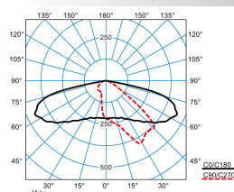
LIQ 50N-AB2L-SLR1/6800-730 6G1 ET (CLO initial value)
