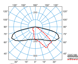
LIQ 50N-AB2L-SLR1/6800-730 6G1 ET (CLO end value)
