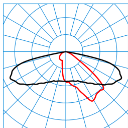
LIQ 50N-AB2L-LRA/6800-727 6G1 ETDD (CLO initial value) TX774767
