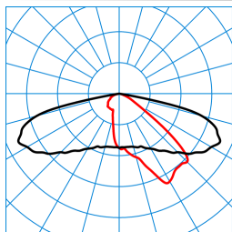
LIQ 50N-AB2L-LRA/6800-727 6G1 ETDD (CLO end value) TX774765
