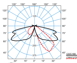
CS 19 100-AB2C/5100-730 4G1 ETDD (CLO end value)
