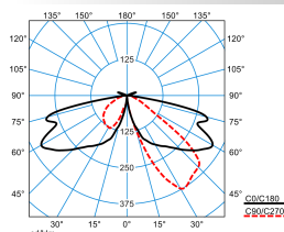
CS 19 100-AB2C/5100-730 4G1 ETDD (CLO initial value)
