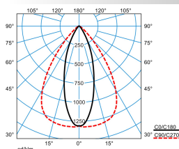
ELINE HE LVN60 827 L150 2 20
