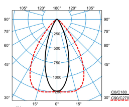
ELINE HE LVN60 865 L150 3 20
