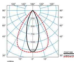
ELINE HE LVN60 840 L150 4 20
