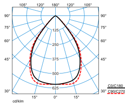
LPCV 3P2-ST L-W 05 45-8TW S96 ETBLE 01 (DCW)
