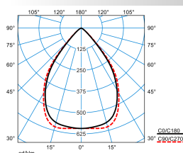
LPCV 3P2-ST L-W 05 45-8TW S96 ETBLE 01 (DWW)
