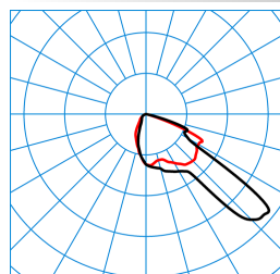
LIQ 70N-FR1L/9100-730 10G1 ET(CLO end value) TX277835 ■ C0 - C180 ■ C90 - C270 DIN 5040: A40 UTE: 1,00 F DLOR: 100 % ULOR: 0 % CEN Flux Code: 41 83 99 100 100
