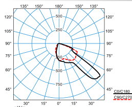
LIQ 70N-FR1L/9100-730 10G1 ET(CLO initial value)
