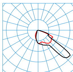
LIQ 70N-FR1L/9100-730 10G1 ET(CLO initial value) TX277748 ■ C0 - C180 ■ C90 - C270 DIN 5040: A40 UTE: 1,00 F DLOR: 100 % ULOR: 0 % CEN Flux Code: 41 83 99 100 100
