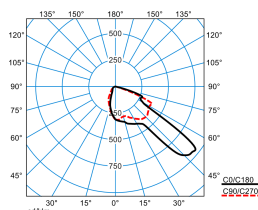
LIQ 70N-FR1L/9100-730 10G1 ET(CLO end value)
