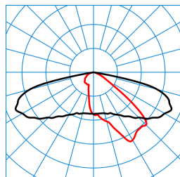
LIQ 50N-AB2L-LR/1500-730 2G1 ET (CLO end value) TX777376 ■ C0 - C180 ■ C90 - C270 DIN 5040: A30 UTE: 1,00 G DLOR: 100 % ULOR: 0 % CEN Flux Code: 34 71 96 100 100 0 0 0 0
