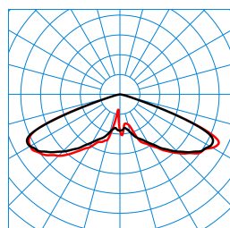
Publisca P2-RB6L/2400-730 3G1S ETDD (CLO end value) TX300178 ■ C0 - C180 ■ C90 - C270 DIN 5040: A20 UTE: 1,00 J DLOR: 100 % ULOR: 0 % CEN Flux Code: 20 57 98 100 100
