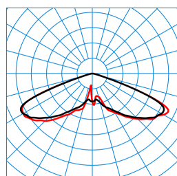
Publisca P2-RB6L/2400-730 3G1S ETDD (CLO initial value) TX300803 ■ C0 - C180 ■ C90 - C270 DIN 5040: A20 UTE: 1,00 J DLOR: 100 % ULOR: 0 % CEN Flux Code: 20 57 98 100 100
