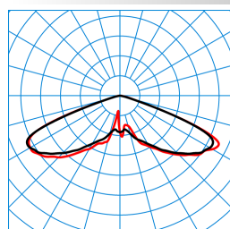
Publisca P2-RB6L/2400-730 3G1S TX047823 ■ C0 - C180 ■ C90 - C270 DIN 5040: A20 UTE: 1,00 J DLOR: 100 % ULOR: 0 % CEN Flux Code: 20 57 98 100 100
