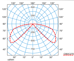
Skeo Q-B1-50-2 AM8R/700-730 1G1P ET TX779617
