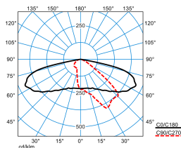
LIQ 50N-AB2L-SLR1/2200-722 2G1 ET (CLO end value)
