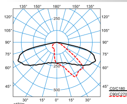
LIQ 50N-AB2L-SLR1/2200-722 2G1 ET (CLO end value) TX776953
