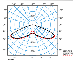
Publisca P2-RB6L/5100-730 6G1S ETDD (CLO initial value)
