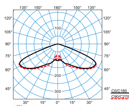
Publisca P2-RB6L/5100-730 6G1S ETDD (CLO end value)
