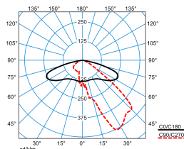
Publisca P2-AB2L/3500-730 4G1S ETDD (CLO initial value) TX300617 DIN 5040: A30 UTE: 1,00 G DLOR: 100 % ULOR: 0 % CEN Flux Code: 35 73 97 100 100
