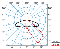
Publisca P2-AB2L/3500-730 4G1S ETDD (CLO end value) TX300559 DIN 5040: A30 UTE: 1,00 G DLOR: 100 % ULOR: 0 % CEN Flux Code: 35 73 97 100 100
