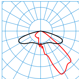
Publisca P2-AB2L/3500-730 4G1S ETDD (CLO initial value) TX300617 ■ C0 - C180 ■ C90 - C270 DIN 5040: A30 UTE: 1,00 G DLOR: 100 % ULOR: 0 % CEN Flux Code: 35 73 97 100 100
