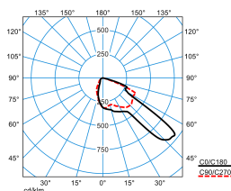
LIQ 50N-FR1L/5600-722 6G1 ET (CLO initial value) TX780628
