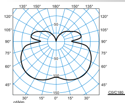
PolaroniQ H2D LED2000-840 ETDD 1,0m
