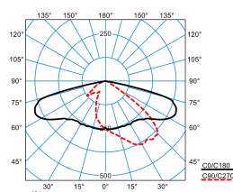
LIQ 70N-AB7L-LRA/75/82/91-740 10G1 ETDD(CLO end value)
