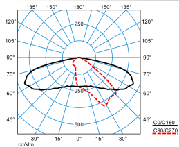
LIQ 50N-AB2L-LR/1650-722 2G1 ET (CLO initial value)
