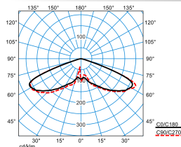
Publisca P2-RB6L/2200-730 3G1S TX047821 DIN 5040: A20 UTE: 1,00 J DLOR: 100 % ULOR: 0 % CEN Flux Code: 20 57 98 100 100
