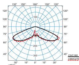
Publisca P2-RB6L/2200-730 3G1S ETDD (CLO initial value) TX301276 DIN 5040: A20 UTE: 1,00 J DLOR: 100 % ULOR: 0 % CEN Flux Code: 20 57 98 100 100
