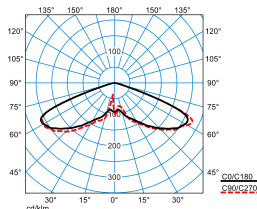
Publisca P2-RB6L/2200-730 3G1S ETDD (CLO end value)
