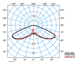
Publisca P2-RB6L/2200-730 3G1S ETDD (CLO end value) TX301436 DIN 5040: A20 UTE: 1,00 J DLOR: 100 % ULOR: 0 % CEN Flux Code: 20 57 98 100 100
