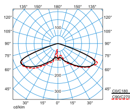
Publisca P2-RB6L/2200-730 3G1S ETDD (CLO initial value)
