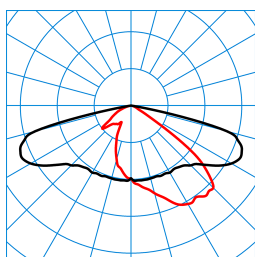
LIQ 70N-AB7L-LR/100/120/135-740 12G1 ET (CLO initial value) TX278350 ■ C0 - C180 ■ C90 - C270 DIN 5040: A30 UTE: 1.00 E DLOR: 100 % ULOR: 0 % CEN Flux Code: 39 76 98 100 100
