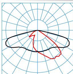
LIQ 70N-AB7L-LR/100/120/135-740 12G1 ET (CLO end value) TX277903 ■ C0 - C180 ■ C90 - C270 DIN 5040: A30 UTE: 1.00 E DLOR: 100 % ULOR: 0 % CEN Flux Code: 39 76 98 100 100
