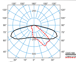
LIQ 50N-AB2L-LR/2000-730 2G1 ET (CLO initial value)
