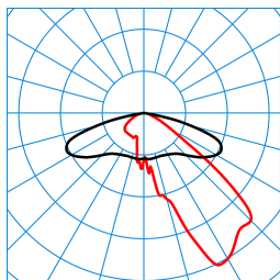
Publisca P2-AB2L/3500-740 4G1S ETDD (CLO initial value) TX301244 ■ C0 - C180 ■ C90 - C270 DIN 5040: A30 UTE: 1,00 G DLOR: 100 % ULOR: 0 % CEN Flux Code: 35 73 97 100 100
