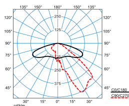
Publisca P2-AB2L/3500-740 4G1S ETDD (CLO initial value) TX301244 DIN 5040: A30 UTE: 1,00 G DLOR: 100 % ULOR: 0 % CEN Flux Code: 35 73 97 100 100
