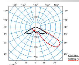
LnPlus 40-AM19L/6200-727 12G1 ETDD (CLO initial value)
