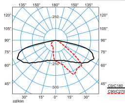
LIQ 50N-AB2L-LRA/5100-727 6G1 ETDD (CLO end value) TX779184
