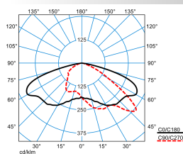
LnPlus 40-AB7L/2200-740 2G1 ETDD (CLO initial value)
