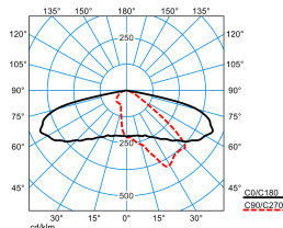
LIQ 50N-AB2L-LRA/5600-727 6G1 ETDD (CLO initial value)
