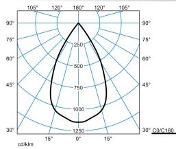
E-Line PRO 78 BV G2 RF-VFL 50-840 M35 ETBLE 03 Blank
