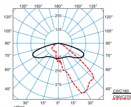
Publisca P2-AB2L/3200-730 4G1S ETDD (CLO initial value) TX301000 DIN 5040: A30 UTE: 1,00 G DLOR: 100 % ULOR: 0 % CEN Flux Code: 35 73 97 100 100
