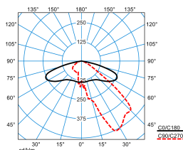
Publisca P2-AB2L/3200-730 4G1S ETDD (CLO end value) TX300339 DIN 5040: A30 UTE: 1,00 G DLOR: 100 % ULOR: 0 % CEN Flux Code: 35 73 97 100 100
