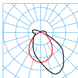
TugraHE Act 18 PAW 64-840 ETDD8 01 (ACTDCW) TX303636 ■ C0 - C180 ■ C90 - C270 DIN 5040: B40 UTE: 0.87 E + 0.13 T DLOR: 87 % ULOR: 13 % CEN Flux Code: 48 79 93 87 100 7 25 60 13
