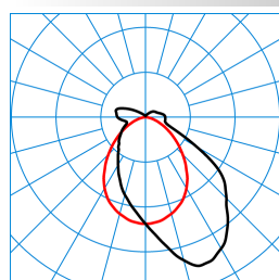
TugraHE Act 18 PAW 64-840 ETDD8 01 (ACTDWW) TX303332 ■ C0 - C180 ■ C90 - C270 DIN 5040: B40 UTE: 0.87 E + 0.13 T DLOR: 87 % ULOR: 13 % CEN Flux Code: 48 79 93 87 100 7 25 60 13
