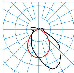
TugraHE Act 18 PAW 64-840 ETDD8 01 (ACTDSU) TX303330 ■ C0 - C180 ■ C90 - C270 DIN 5040: B40 UTE: 0.87 E + 0.13 T DLOR: 87 % ULOR: 13 % CEN Flux Code: 48 79 93 87 100 7 25 60 13
