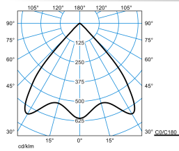
Inveria C 210 RB22R/3100-830 1G1P ET
