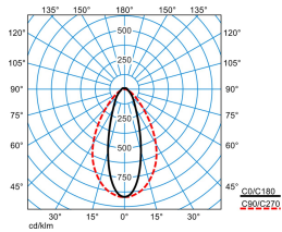
ELINE HE PN140 865 L225 1 20
