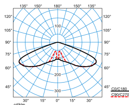
Publisca P2-RB6L/1000-740 2G1S ETDD (CLO end value)
