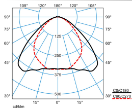
ELINE HE+ LVW160 830 L225 1 20
