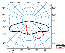
LIQ 70N-AB7L-LRA/75/82/91-730 10G1 ETDD(CLO initial value) TX278058
