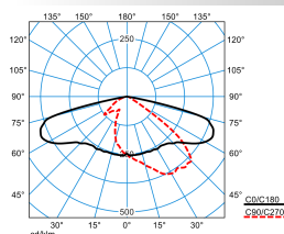
LIQ 70N-AB7L-LRA/75/82/91-730 10G1 ETDD(CLO end value) TX277840
