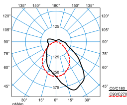
TugraHE 15 PAW 28-89/16ML-830 ET PC 23 (stage 4)
