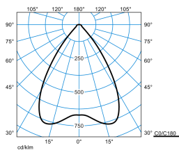
InperiaL G2 C07 BR19 2700-840 01 + ZN-PC TX052850
