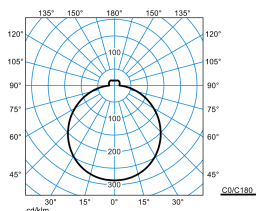
Solegra D3 OTA 13500-830 + ZS A 3075/3000 TX772752
