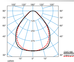
ArimoFit M46 PW19 42-8TW ETDD8 (DCW)
