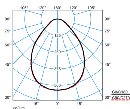
ArimoFit M46 PW19 42-8TW ETDD8 + ArimoFit Sky M46-TS ZER (DCW)
