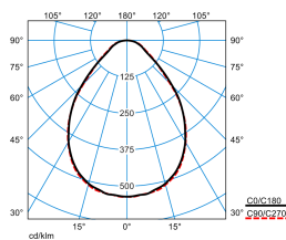
ArimoFit M46 PW19 42-8TW ETDD8 + ArimoFit Sky M46-TS ZER (DWW)
