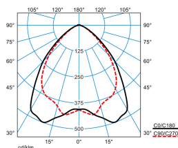
ELINE LW40-110 ML 865 L150 4 20
