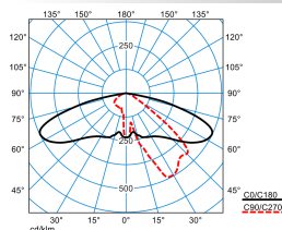
Publisca P2-AB2L/5100-730 6G1S ETDD (CLO initial value)
