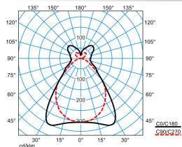
ELINE HE PMW2290 840 L150 1 50
