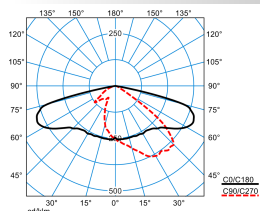
LIQ 70N-AB7L-SLR1/9100-740 10G1 ET(CLO end value) TX278179
